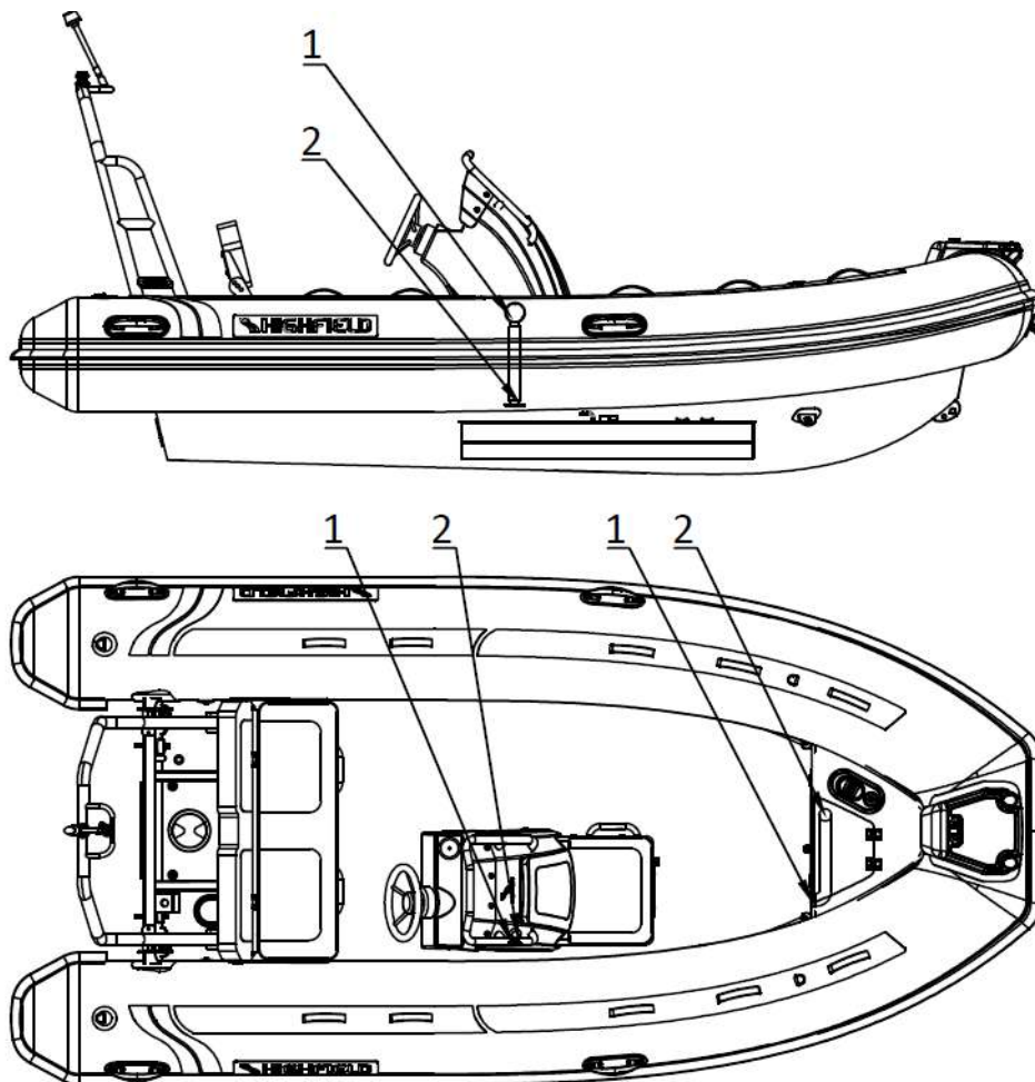
Diagram of the layout- Ventilation of petrol tank compartment (CL420-460)
